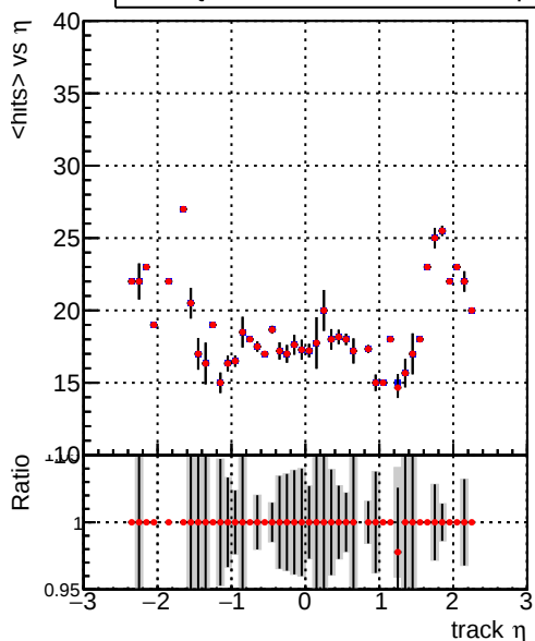
mean hit — DQM_mkFit5_TT_retrainOldFiles125_v2_prelimWP_epoch4
