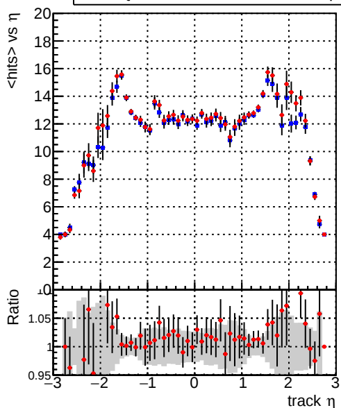
mean hits vs \eta Legend: DQM_mkFit_TTbase (blue line), DQM_mkFit5_TT_retrainOldFiles125_v2_prelimWP_epoch4 (red line)
