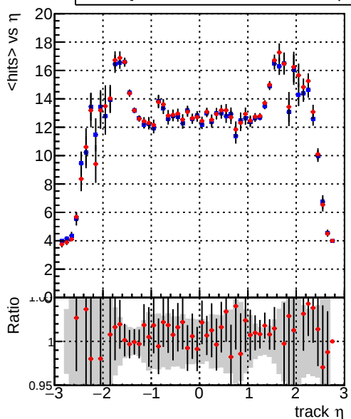
— DQM_mkFit_TTbase — DQM_mkFit5_TT_retrainOldFiles125_v2_prelimWP_epoch4 mean hit
