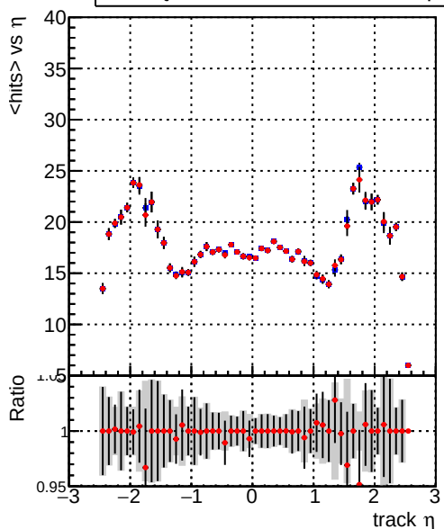
mean hits vs \eta Legend: DQM_mkFit5_TTbase (blue line), DQM_mkFit5_TT_retrainOldFiles125_v2_prelimWP_epoch4 (red line)
