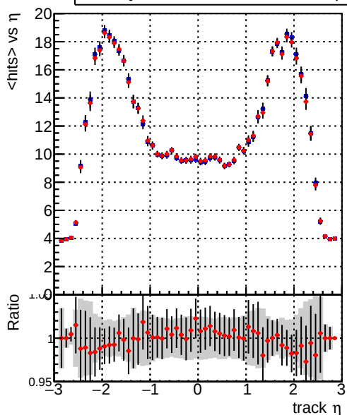
mean hits vs \eta — DQM_mkFit5_TT_retrainOldFiles125_v2_prelimWP_epoch4
