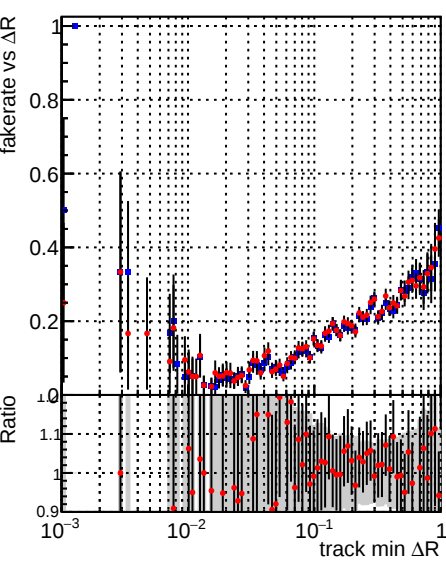
Legend: DQM_mkFit_TTbase (blue squares), DQM_mkFit5_TT_retrainOldFiles125_v2_prelimWP_epoch4 (red circles)
