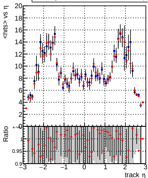
— DQM_mkFit5_TTbase — DQM_mkFit5_TT_retrainOldFiles125_v2_prelimWP_epoch4 mean hits vs \eta
