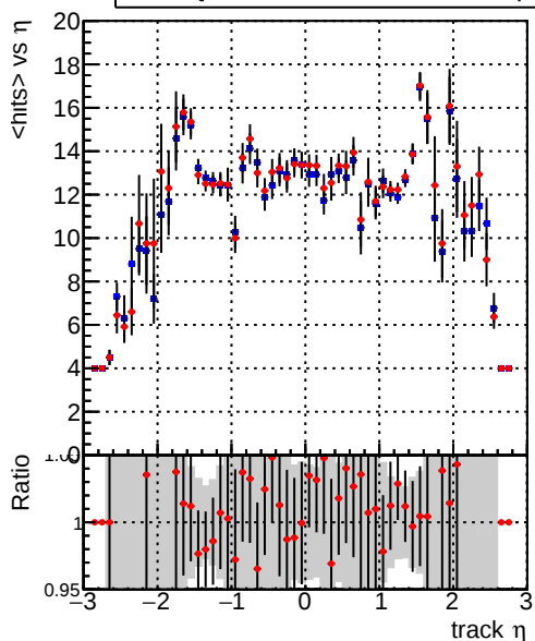
mean hit — DQM_mkFit5_TTbase — DQM_mkFit5_TT_retrainOldFiles125_v2_prelimWP_epoch4
