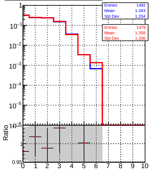
mean hit \eta Legend: DQM_mkFit5_TTbase (blue line), DQM_mkFit5_TT_retrainOldFiles125_v2_prelimWP_epoch4 (red line)
