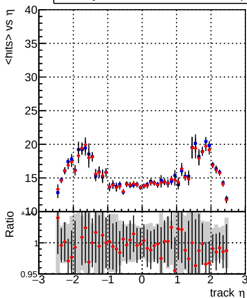
mean hit \eta Legend: DQM_mkFit5_TTbase (blue line), DQM_mkFit5_TT_retrainOldFiles125_v2_prelimWP_epoch4 (red line)
