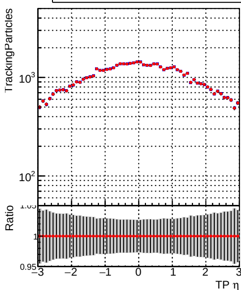
N of simulated tracks vs \eta Legend: ■ DQM_mkFit_TTbase ■ DQM_mkFit5_TT_retrainOldFiles125_v2_prelimWP_epoch4
