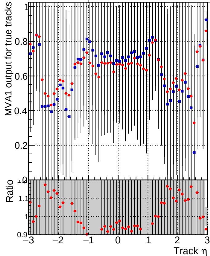
MVA1 of associated tracks (recoToSim) vs. track \eta Legend: DQM_mkFit_TTbase (blue squares) DQM_mkFit5_TT_retrainOldFiles125_v2_prelimWP_epoch4 (red diamonds)
