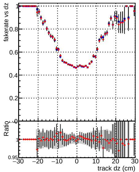
Fake rate vs dz —●— DQM_mkFit_TTbase —●— DQM_mkFit5_TT_retrainOldFiles125_v2_prelimWP_epoch4
