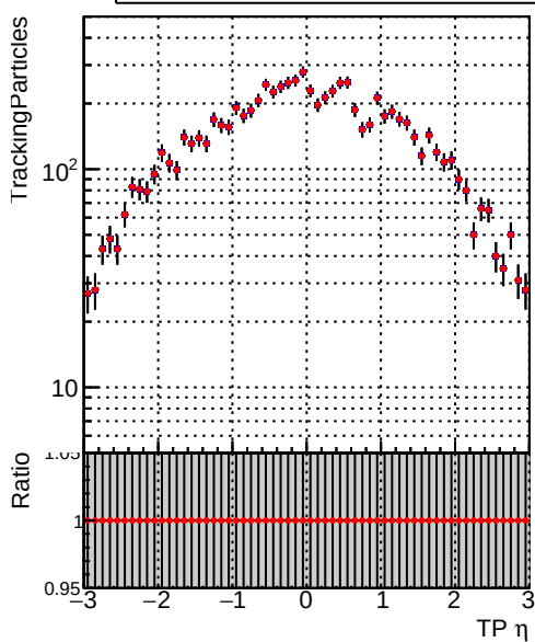
N of simulated tracks vs \eta Legend: DQM_mkFit_TTbase (blue square), DQM_mkFit5_TT_retrainOldFiles125_v2_prelimWP_epoch4 (red circle)
