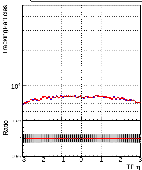
N of simulated tracks vs TP \eta —•— DQM_mkFit_TTbase —•— DQM_mkFit5_TT_retrainOldFiles125_v2_prelimWP_epoch4
