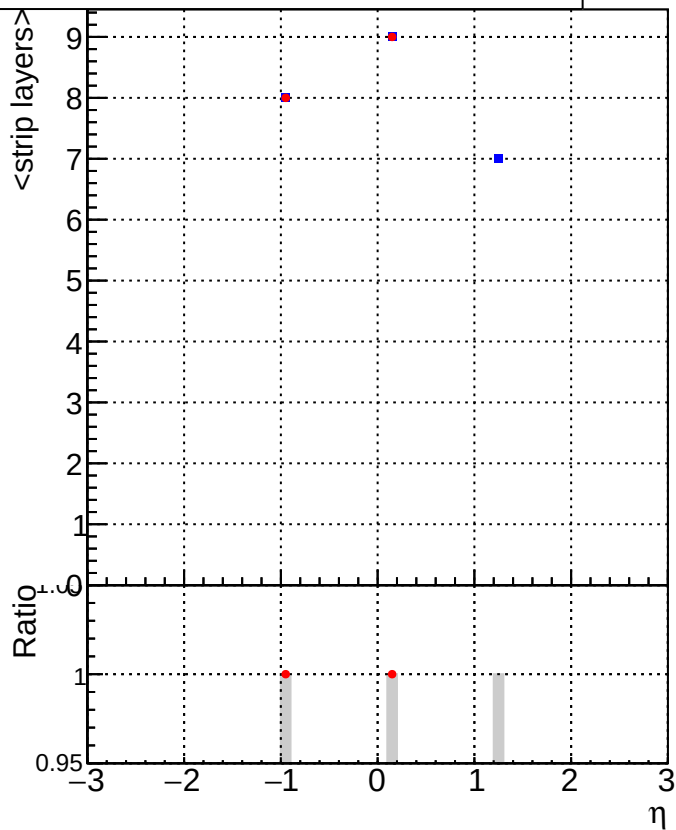
Legend: DQM_mkFit_TTbase (blue square) DQM_mkFit5_TT_retrainOldFiles125_v2_prelimWP_epoch4 (red square)
