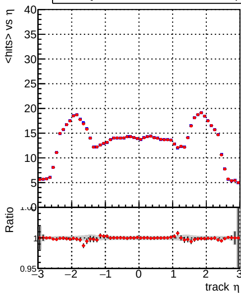
mean hit \eta Legend: DQM_mkFit5_TT_retrainOldFiles125_v2_prelimWP_epoch4 (red line), DQM_mkFit5_TTbase (blue line)
