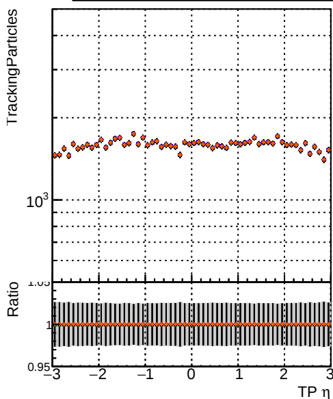
N of simulated tracks vs \eta Legend: DQM_mkFit_TTbase DQM_mkFit5_TT_retrainOldFiles125_v2_prelimWP_epoch4 DQM_mkFit_TT_baseline_6iter DQM_mkFit6_TT_retrainOldFiles125_v2_prelimWP_epoch2_wSQCD
