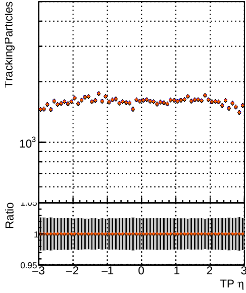
—●— DQM_mkFit_TTbase —●— DQM_mkFit5_TT_retrainOldFiles125_v2_prelimWP_epoch4 —●— DQM_mkFit6_TT_baseline_6iter —●— DQM_mkFit6_TT_retrainOldFiles125_v2_prelimWP_epoch2_wsQCD
