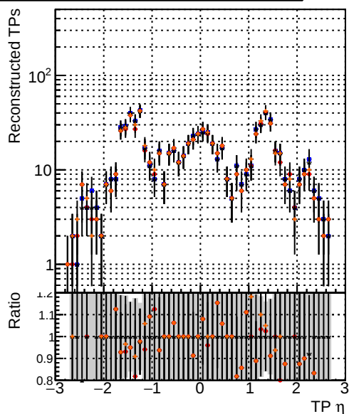
—•— DQM_mkFit_TTbase —•— DQM_mkFit5_TT_retrainOldFiles125_v2_prelimWP_epoch4 —•— DQM_mkFit_TT_baseline_6iter —•— DQM_mkFit6_TT_retrainOldFiles125_v2_prelimWP_epoch2_wsQCD
