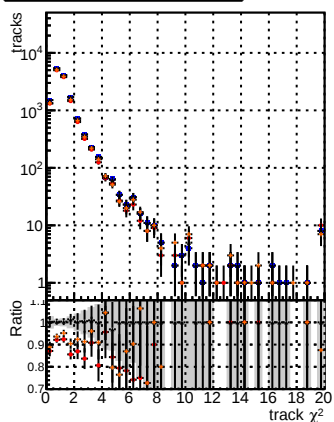
N of reco track vs. \chi^2 for BSM mFit TTbase, BSM mFit TTbase + L1 base, and BSM mFit TTbase + L1 + base. The legend indicates the models used for the plots.
