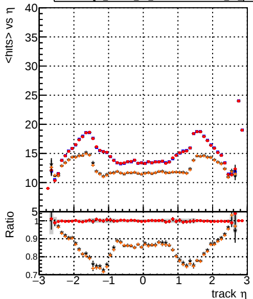
mean hits > \eta — DQM_mkFit_TTbase — DQM_mkFit5_TT_retrainOldFiles125_v2_prelimWP_epoch4 — DQM_mkFit_TT_baseline_6iter — DQM_mkFit6_TT_retrainOldFiles125_v2_prelimWP_epoch2_wsQCD
