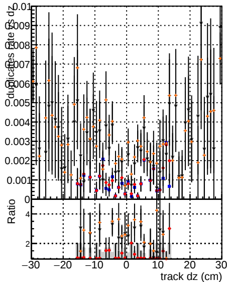
Legend: - \square DQM mkFit TTbase - \square DQM mkFit TTbase + 15.11.2019 OldFiles125_v2_prelimWP_epoch4 - \square DQM mkFit TTbase + 15.11.2019 OldFiles125_v2_prelimWP_epoch2_wSQCD
