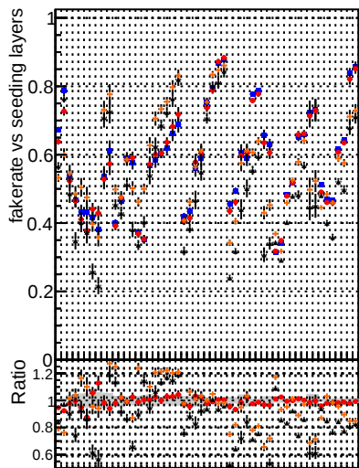
Fake rate vs. ● DGM mkFit TTbase ★ DGM mkFit TTbase+15 ★ DGM mkFit TTbase+16 ★ DGM mkFit TTbase+16+17 ■ DGM mkFit TTbase+15+16+17+18+19+20+21+22+23+24+25+26+27+28+29+30+31+32+33+34+35+36+37+38+39+40+41+42+43+44+45+46+47+48+49+50+51+52+53+54+55+56+57+58+59+60+61+62+63+64+65+66+67+68+69+70+71+72+73+74+75+76+77+78+79+80+81+82+83+84+85+86+87+88+89+90+91+92+93+94+95+96+97+98+99+100
