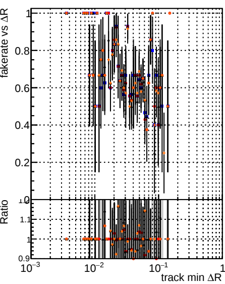
Fake rate vs \Delta R (track, jet) DOM mkFit TTbase retrainOldFiles125_v2_prelimWP_epoch4 DOM mkFit TTbase retrainOldFiles125_v2_prelimWP_epoch2_wSQCD DOM mkFit TTbase retrainOldFiles125_v2_prelimWP_epoch2_wSQCD
