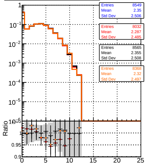
mean hit DQM_mkFit_TTbase DQM_mkFit5_TT_retrainOldFiles125_v2_prelimWP_epoch4 DQM_mkFit_TT_baseline_6iter DQM_mkFit6_TT_retrainOldFiles125_v2_prelimWP_epoch2_wsQCD
