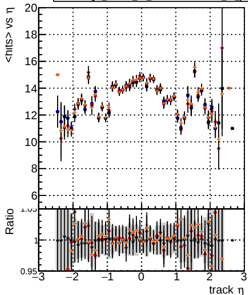
mean hit DQM_mkFit_TTbase DQM_mkFit5_TT_retrainOldFiles125_v2_prelimWP_epoch4 DQM_mkFit_TT_baseline_6iter DQM_mkFit6_TT_retrainOldFiles125_v2_prelimWP_epoch2_wsQCD
