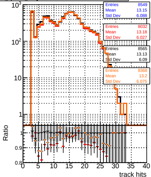
mean hit DQM_mkFit_TTbase DQM_mkFit5_TT_retrainOldFiles125_v2_prelimWP_epoch4 DQM_mkFit_TT_baseline_6iter DQM_mkFit6_TT_retrainOldFiles125_v2_prelimWP_epoch2_wsQCD
