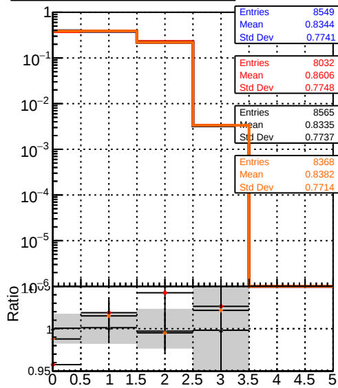
mean hit DQM_mkFit_TTbase DQM_mkFit5_TT_retrainOldFiles125_v2_prelimWP_epoch4 DQM_mkFit_TT_baseline_6iter DQM_mkFit6_TT_retrainOldFiles125_v2_prelimWP_epoch2_wsQCD
