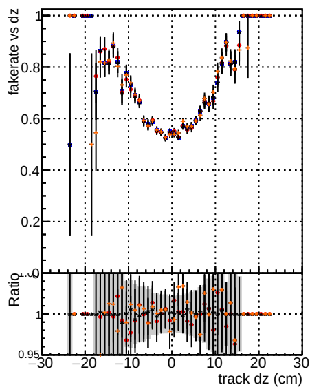
Legend: — DGM mkFit5 TTbase — DGM mkFit5 TTbase125 v2_prelimWP_epoch4 — DGM mkFit6 TTbase125 v2_prelimWP_epoch2_wSQCD
