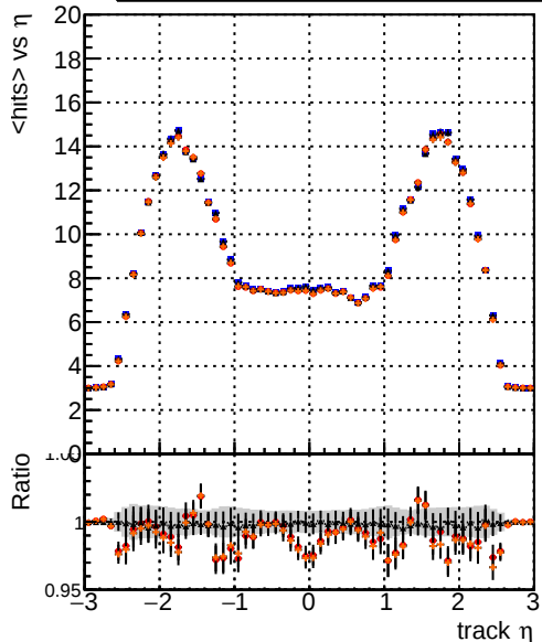
Legend: DQM_mkFit5_TTbase (blue line), DQM_mkFit5_TT_retrainOldFiles125_v2_prelimWP_epoch4 (red line with dots), DQM_mkFit6_TT_baseLine_6iter (black line with dots), DQM_mkFit6_TT_retrainOldFiles125_v2_prelimWP_epoch2_wsQCD (orange line with dots) mean hits > \eta
