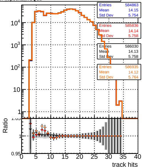
mean hit DOM_mkFit_TTbase DOM_mkFit5_TT_retrainOldFiles125_v2_prelimWP_epoch4 DOM_mkFit6_TT_retrainOldFiles125_v2_prelimWP_epoch2_wsQCD
