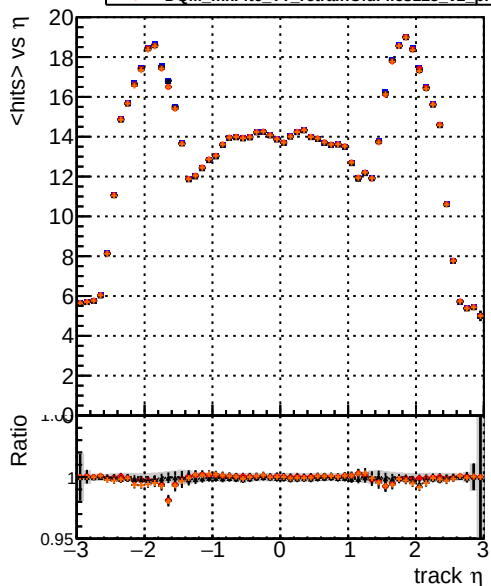
mean hit DOM_mkFit_TTbase DOM_mkFit5_TT_retrainOldFiles125_v2_prelimWP_epoch4 DOM_mkFit6_TT_retrainOldFiles125_v2_prelimWP_epoch2_wsQCD
