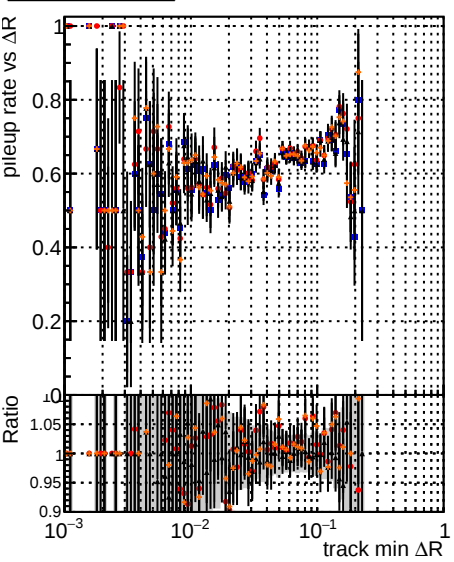
DOM mkFit TTbase DOM mkFit5 TTbase DOM mkFit6 TTbase DOM mkFit6 TT retrainOldFiles125_v2_prelimWP_epoch4 DOM mkFit6 TT retrainOldFiles125_v2_prelimWP_epoch2_wSQCD
