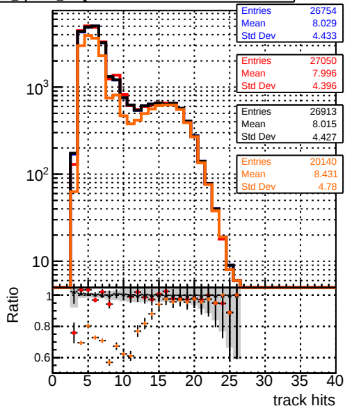
mean hit DQM_mkFit5_TTbase DQM_mkFit5_TT_retrainOldFiles125_v2_prelimWP_epoch4 DQM_mkFit5_TT_baseLine_6iter DQM_mkFit6_TT_retrainOldFiles125_v2_prelimWP_epoch2_wsQCD
