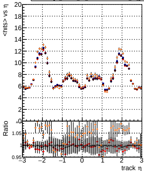
mean hit DQM_mkFit5_TTbase DQM_mkFit5_TT_retrainOldFiles125_v2_prelimWP_epoch4 DQM_mkFit5_TT_baseLine_6iter DQM_mkFit6_TT_retrainOldFiles125_v2_prelimWP_epoch2_wsQCD
