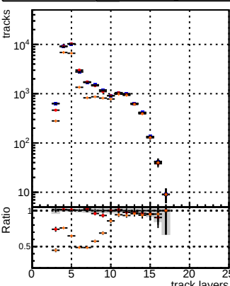
N of reco track vs track layers
