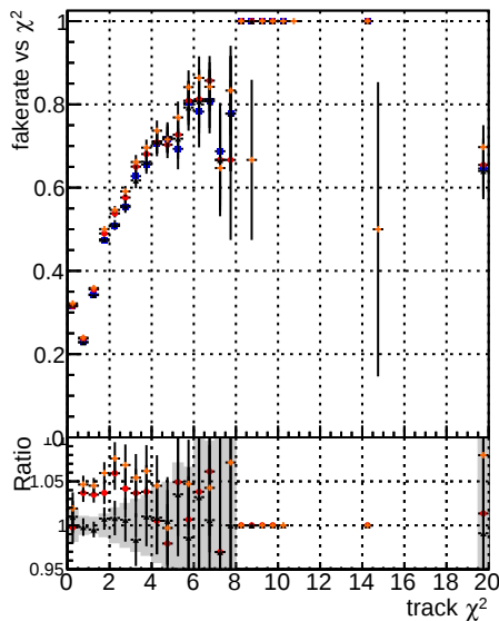
Fake rate vs. DOM mkFit TTbase retrainOldFiles125_v2 prelimWP epoch4 DOM mkFit 15 TT baseLine file DOM mkFit 16 TT retrainOldFiles125_v2 wSQCD
