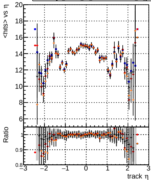
mean hits vs \eta DOM_mkFit5_TTbase DOM_mkFit5_TT_retrainOldFiles125_v2_prelimWP_epoch4 DOM_mkFit6_TT_baseLine_6iter DOM_mkFit6_TT_retrainOldFiles125_v2_prelimWP_epoch2_wsQCD
