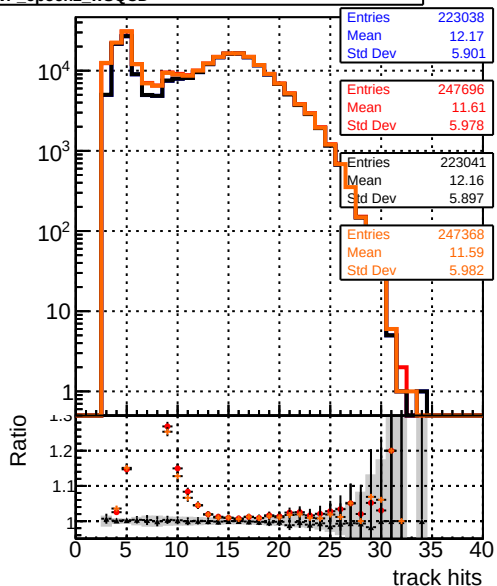
mean hit DOM_mkFit1_TTbase DOM_mkFit5_TT_retrainOldFiles125_v2_prelimWP_epoch4 DOM_mkFit6_TT_baseline_6iter DOM_mkFit6_TT_retrainOldFiles125_v2_prelimWP_epoch2_wsQCD
