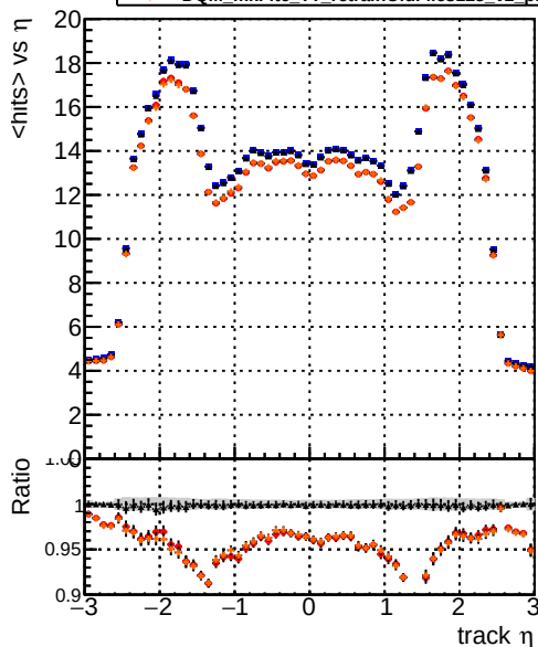
mean hit DOM_mkFit1_TTbase DOM_mkFit5_TT_retrainOldFiles125_v2_prelimWP_epoch4 DOM_mkFit6_TT_baseline_6iter DOM_mkFit6_TT_retrainOldFiles125_v2_prelimWP_epoch2_wsQCD
