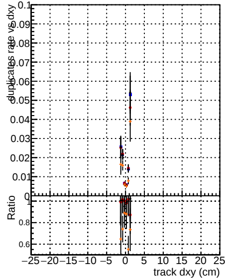
Fake rate vs dz Duplicates Rate vs Dxy Pileup rate vs dxy DGM mkFit TTbase DGM mkFit TTbase DGM mkFit TTbase DGM mkFit TTbase
