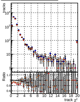
N of reco track vs. \chi^2 for BSM mFit TTbase, BSM mFit TTbase + Lb, and BSM mFit TTbase + Lb + trainOldFiles125 v2_prelimWP_epoch4
