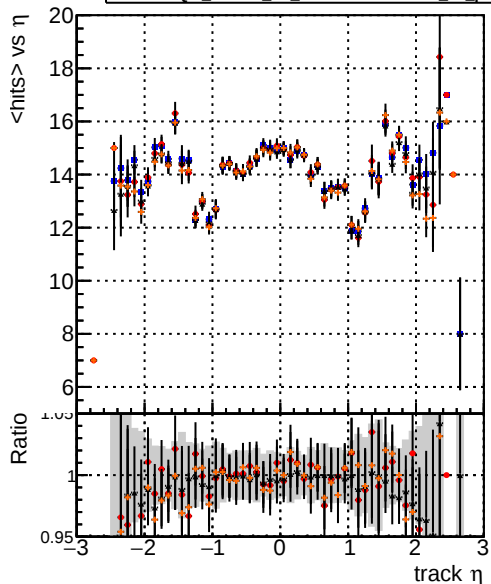
mean hit DQM_mkFit1_TTbase DQM_mkFit5_TT_retrainOldFiles125_v2_prelimWP_epoch4 DQM_mkFit6_TT_retrainOldFiles125_v2_prelimWP_epoch2_wsQCD
