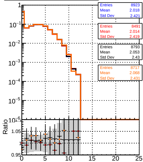
mean hit DQM_mkFit1_TTbase DQM_mkFit5_TT_retrainOldFiles125_v2_prelimWP_epoch4 DQM_mkFit6_TT_retrainOldFiles125_v2_prelimWP_epoch2_wsQCD
