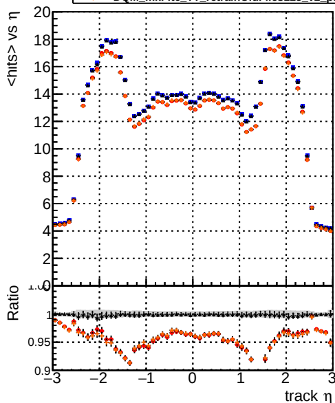
mean hits vs \eta Legend: - DQM_mkFit1_TTbase (blue line) - DQM_mkFit5_TT_retrainOldFiles125_v2_prelimWP_epoch4 (red line with stars) - DQM_mkFit6_TT_retrainOldFiles125_v2_prelimWP_epoch2_wsQCD (orange line with stars)
