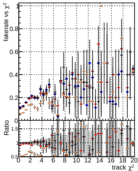
Fake rate vs. Legend: DQM mkFit5 TTbase DQM mkFit6 TTbase DQM mkFit6 TTbase trainOldFiles125_v2_prelimWP_epoch4 trainOldFiles125_v2_prelimWP_epoch2_wsQCD
