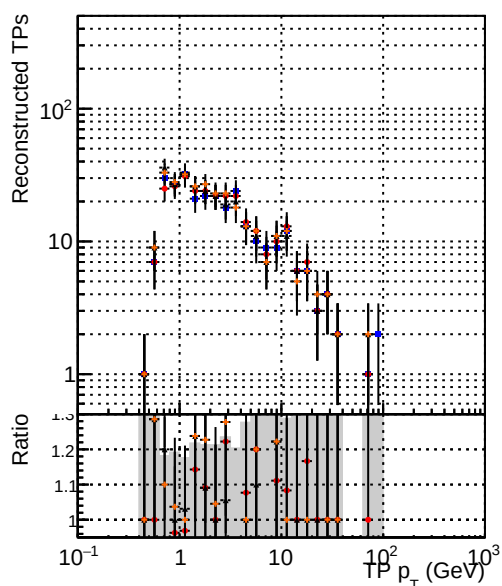
— DQM_mkFit5_TTbase — DQM_mkFit5_TT_retrainOldFiles125_v2_prelimWP_epoch4 — DQM_mkFit6_TT_baseline_6iter — DQM_mkFit6_TT_retrainOldFiles125_v2_prelimWP_epoch2_wsQCD
