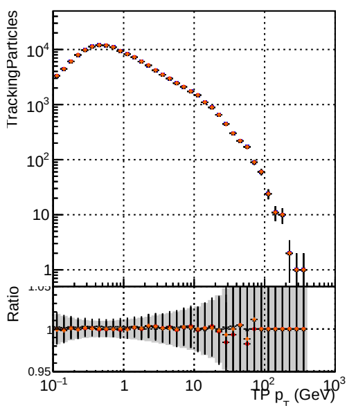
● DQM_mkFit1_TTbase ● DQM_mkFit5_TT_retrainOldFiles125_v2_prelimWP_epoch4 ▲ DQM_mkFit_TT_baseline_6iter ● DQM_mkFit6_TT_retrainOldFiles125_v2_prelimWP_epoch2_wsQCD
