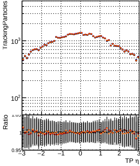
● DQM_mkFit1_TTbase ● DQM_mkFit5_TT_retrainOldFiles125_v2_prelimWP_epoch4 ▲ DQM_mkFit_TT_baseline_6iter ● DQM_mkFit6_TT_retrainOldFiles125_v2_prelimWP_epoch2_wsQCD
