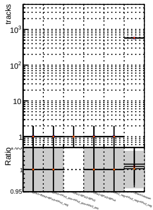
N of reco track vs. \chi^2 BSM mFit TTbase BSM mFit TTbase + L1 baseline BSM mFit TTbase + L1 + RetrainORFiles125 v2_prelimWP_epoch4 BSM mFit TTbase + L1 + RetrainORFiles125 v2_prelimWP_epoch2_wSQCD
