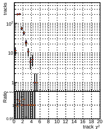
N of reco track vs. \chi^2 BSM mFit TTbase BSM mFit TTbase + L1 baseline BSM mFit TTbase + L1 + RetrainORFiles125 v2_prelimWP_epoch4 BSM mFit TTbase + L1 + RetrainORFiles125 v2_prelimWP_epoch2_wSQCD
