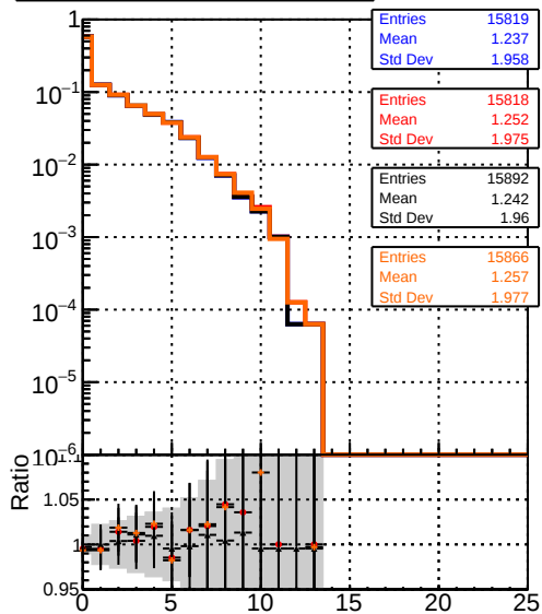
mean hits — DQM_mkFit_TTbase — DQM_mkFit5_TT_retrainOldFiles125_v2_prelimWP_epoch4 — DQM_mkFit6_TT_retrainOldFiles125_v2_prelimWP_epoch2_wsQCD
