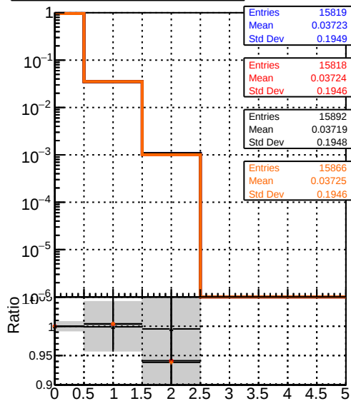
mean hits — DQM_mkFit_TTbase — DQM_mkFit5_TT_retrainOldFiles125_v2_prelimWP_epoch4 — DQM_mkFit6_TT_retrainOldFiles125_v2_prelimWP_epoch2_wsQCD
