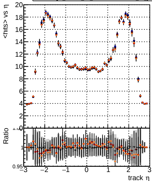
mean hits — DQM_mkFit_TTbase — DQM_mkFit5_TT_retrainOldFiles125_v2_prelimWP_epoch4 — DQM_mkFit6_TT_retrainOldFiles125_v2_prelimWP_epoch2_wsQCD
