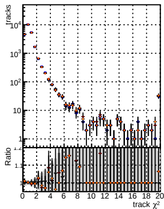
N of reco track vs. \chi^2 for BSM mFit + base + retainOR Files125 v2_prelimWP_epoch4
