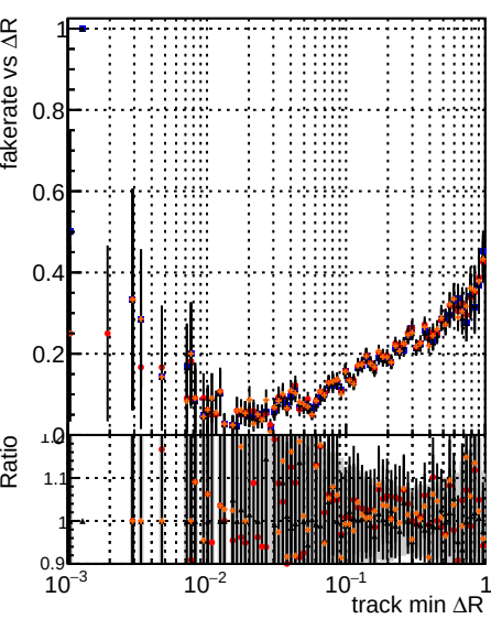
Fake rate vs \Delta R(\text{track, jet}) DQM mkFit TTbase retrainOldFiles125_v2_prelimWP_epoch4 DQM mkFit5 TTbase retrainOldFiles125_v2_prelimWP_epoch2 wSQCD DQM mkFit6 TTbase retrainOldFiles125_v2_prelimWP_epoch2 wSQCD
