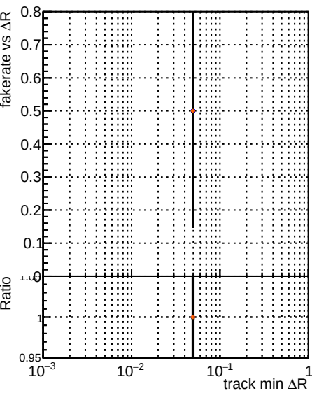
Fake rate vs \Delta R(\text{track, jet}) DOM mktFit TTbase retrainOldFiles125_v2_prelimWP_epoch4 DOM mktFit5 TTbase retrainOldFiles125_v2_prelimWP_epoch2 DOM mktFit6 TTbase retrainOldFiles125_v2_prelimWP_epoch2_wSQCD
