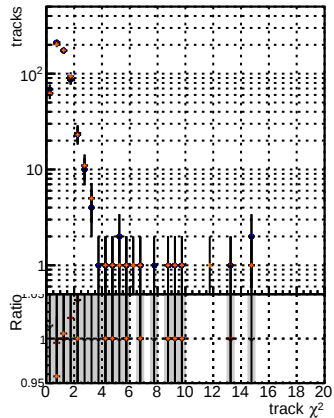
N of reco track vs. \chi^2 for BGM, mFit, TTree, and Baseline. The legend indicates the models used in the plots.
