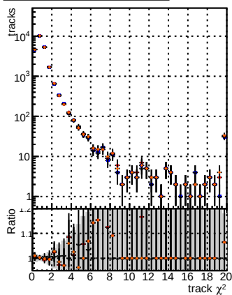
N of reco track vs. \chi^2 for BSM mFit + base + retainOR Files125 v2_prelimWP_epoch4 (blue), BSM mFit + base + retainOR Files125 v2_prelimWP_epoch2 (orange), and BSM mFit + base + retainOR Files125 v2_prelimWP_epoch2 wSQCD (red)
