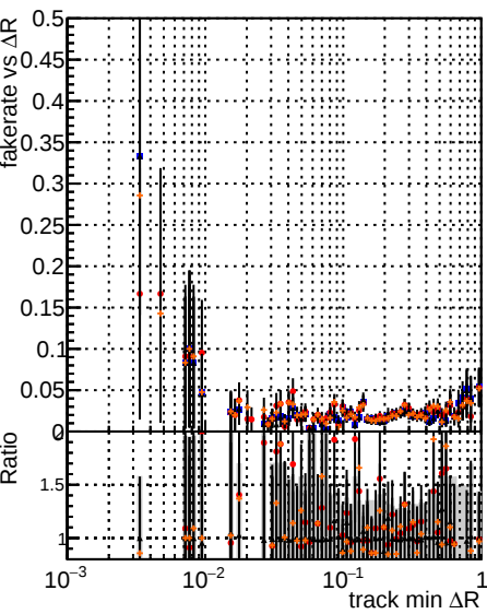
Fake rate vs ΔR(track, jet) DOM mkFit TTbase DOM mkFit5 TTbase DOM mkFit6 TTbase DOM mkFit TT retrainOldFiles125_v2_prelimWP_epoch4 DOM mkFit TT retrainOldFiles125_v2_prelimWP_epoch2_wSQCD
