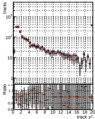
N of reco track vs. \chi^2 for BSM mFit v2 (black), BSM mFit v2 wSQCD (red), BSM mFit v2 wSQCD (blue), and BSM mFit v2 wSQCD (orange). The legend also includes BSM mFit v2 wSQCD (black), BSM mFit v2 wSQCD (red), BSM mFit v2 wSQCD (blue), and BSM mFit v2 wSQCD (orange).
